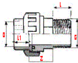
RACCORD UNION 3 P. FEMELLE A COLLER - MALE A VISER
